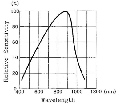
Spectral Sensitivity
