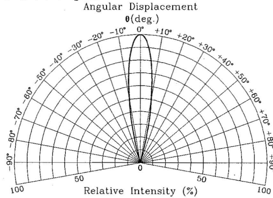
Radiation Diagram
